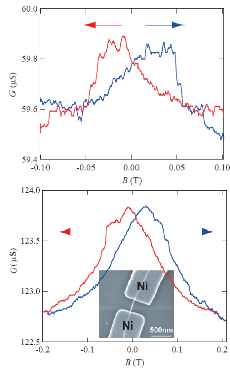
Spin injection
