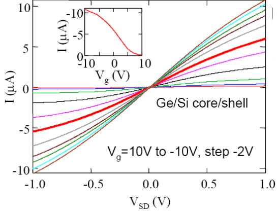
Clean Ge channel with Ohmic contacts
