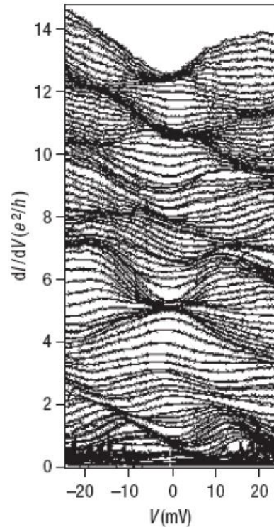
1D transport
