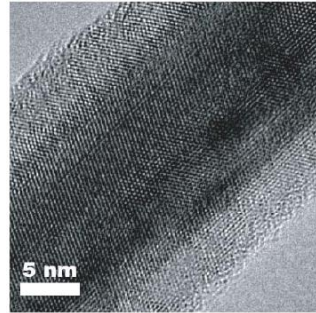
Spin injection
