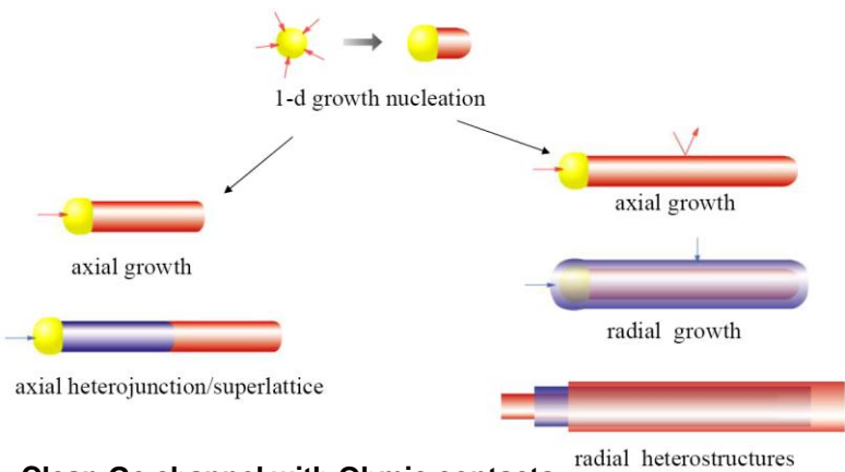
1D transport
